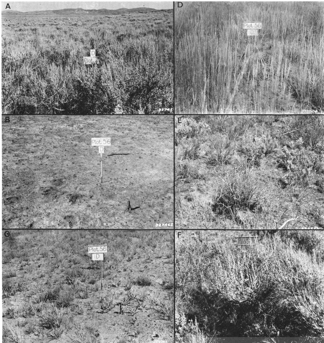
Fig. 4. Plot depicting vegetation changes in sagebrush-grass range after a planned burn: (a) 1936 (before burning), sagebrush cover extremely dense, grass and forbs unavailable for grazing; (b) 1936 (after burning), complete removal of sagebrush-grass vegetation; (c) 1937, return of forbs and grasses with little brush apparent; (d) 1938, excellent grass and forbs stand with little brush apparent; (e) 1948, grass and forbs readily available to grazing intermixed with a few shrubs; (f) 1966, return of dense sagebrush cover and unavailable understory of grass and forbs.
