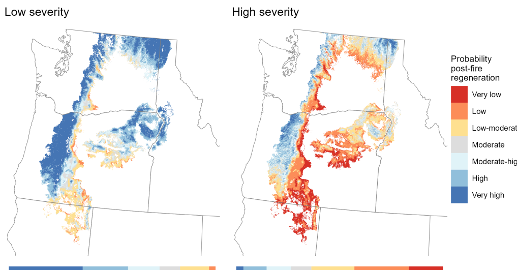
Figure 3. Projected probability of post-fire regeneration under a future climate scenario (2031-2050; moderate emissions RCP 4.5) and either low severity (left) or high severity (right) fire scenarios for all study species combined. In the low severity scenario the nearest seed source is 10 m away, while in the high severity scenario it is 150 m away.
