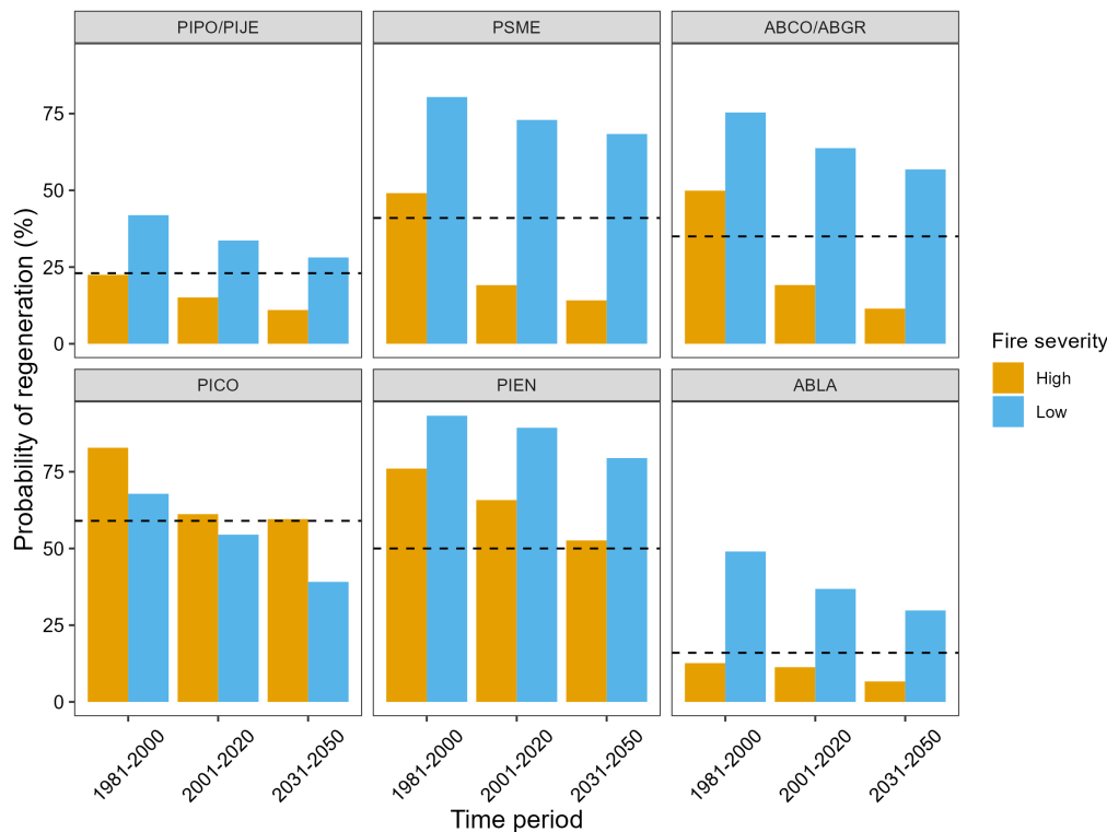
Figure 4. Median probability of post-fire regeneration for individual species across the range of each species within the Interior Northwest region (Fig. 1). The dashed black line is the threshold probability above which regeneration is likely (which varies by species). “PIPO/PIJE” is ponderosa/Jeffrey pine; “PSME” is Douglas-fir; “ABCO/ABGR” is white/grand fir; “PICO” is lodgepole pine; “PIEN” is Engelmann spruce; “ABLA” is subalpine fir.
