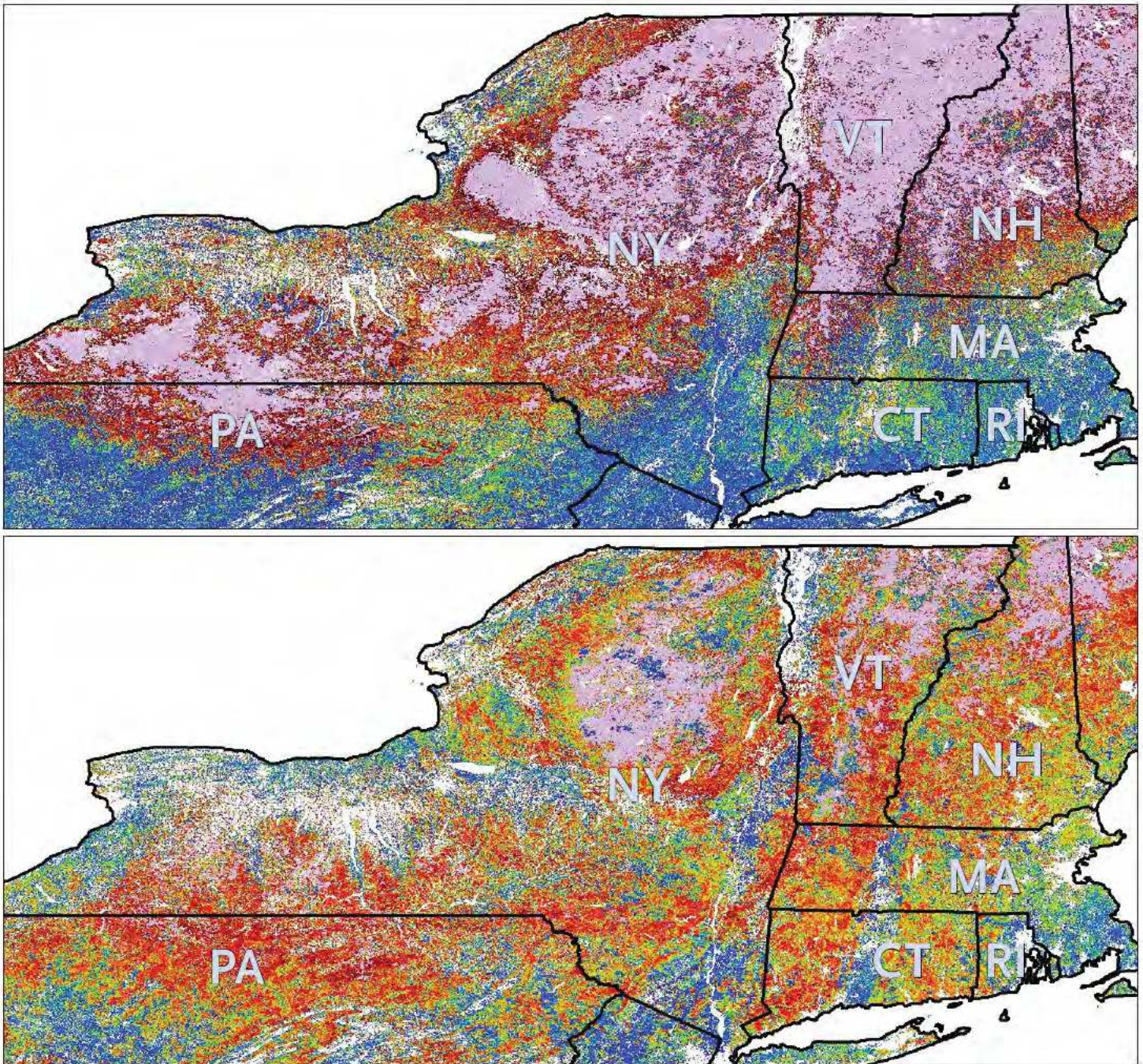
Figure 5—In late March 2011 (top), extensive snow cover remained in the higher elevations of the Northeast and contributed to lower than average levels of forest vigor. Five weeks later, by early May (bottom), snow still lingered in the Adirondacks and northern New England, as shown in pink and dark red; spring greenup was still delayed over extensive portions of the Northeast relative to the 8-year historical baseline, as shown in red, orange, and yellow.
